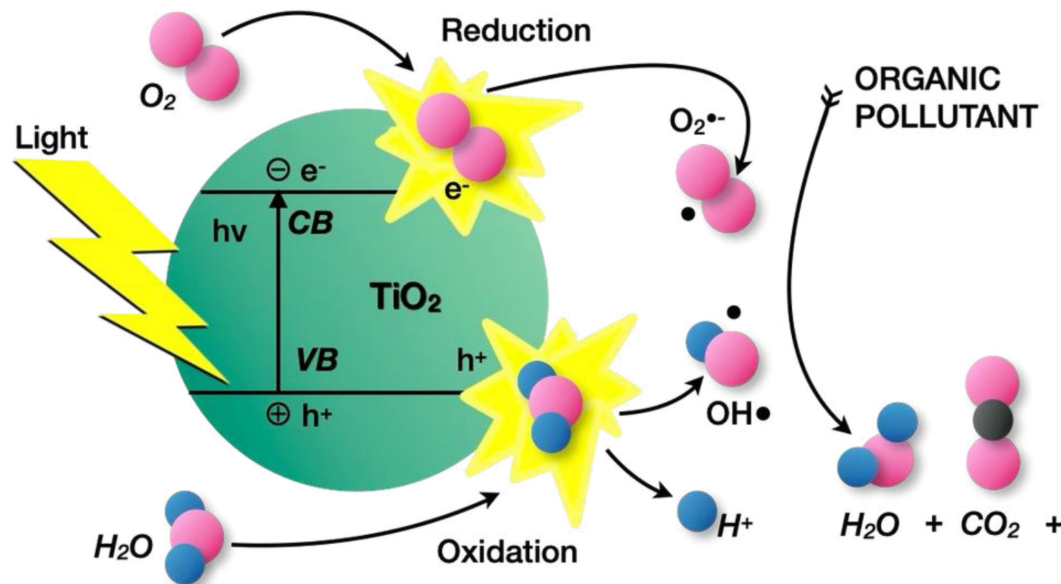
Figure 1. Schematic of semiconductor excitation by band gap illumination leading to the creation of “electrons” in the conduction band and “holes” in the valence band.
